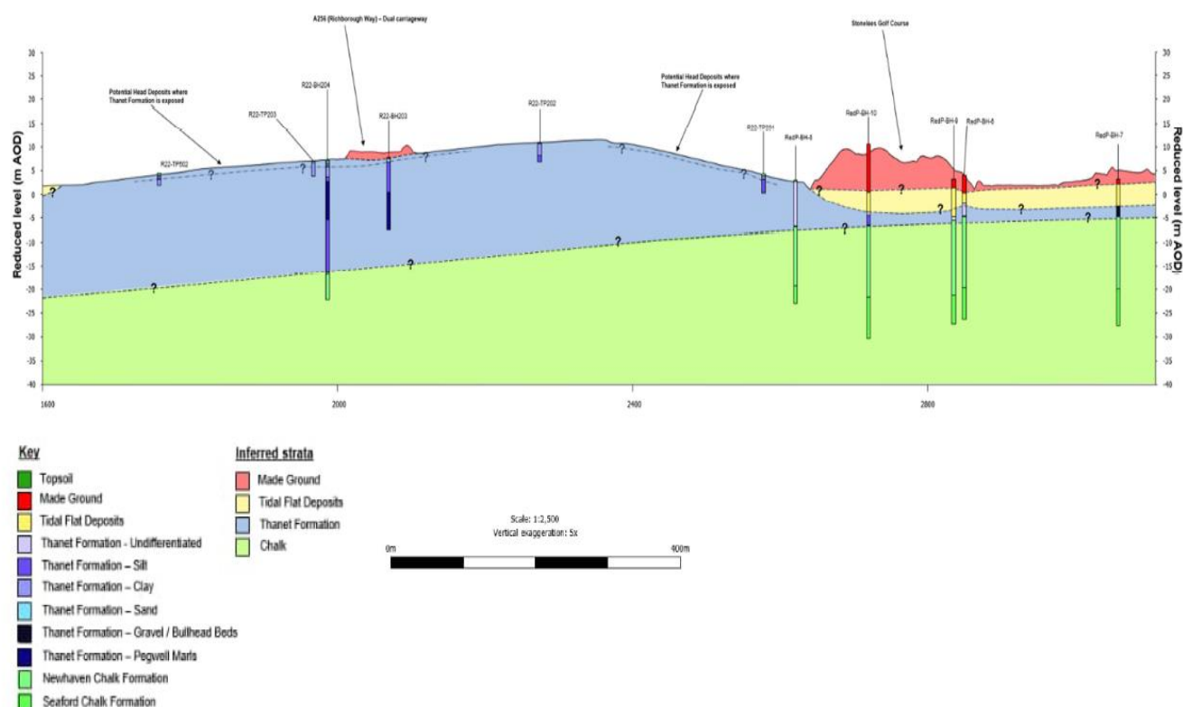
Figure B.4: Sketch geological section – Sheet 2
